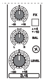
Fig. 2.6: Le manopole FX send/balance/level
