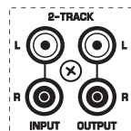
Fig. 2.11: Tape input/output
