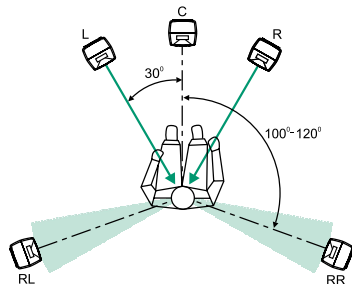
Figure 2. Correct alignment of the loudspeakers in a 5-channel system.
