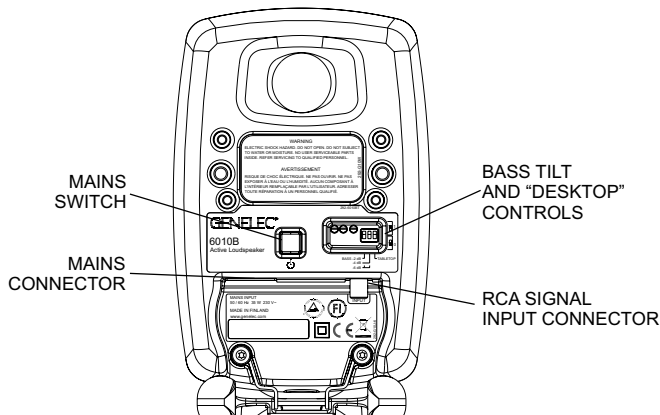
Figure 3. Control and connector layout on the rear panel of a 6010B.
