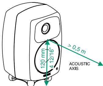
Figure 1. Location of the acoustic axis
